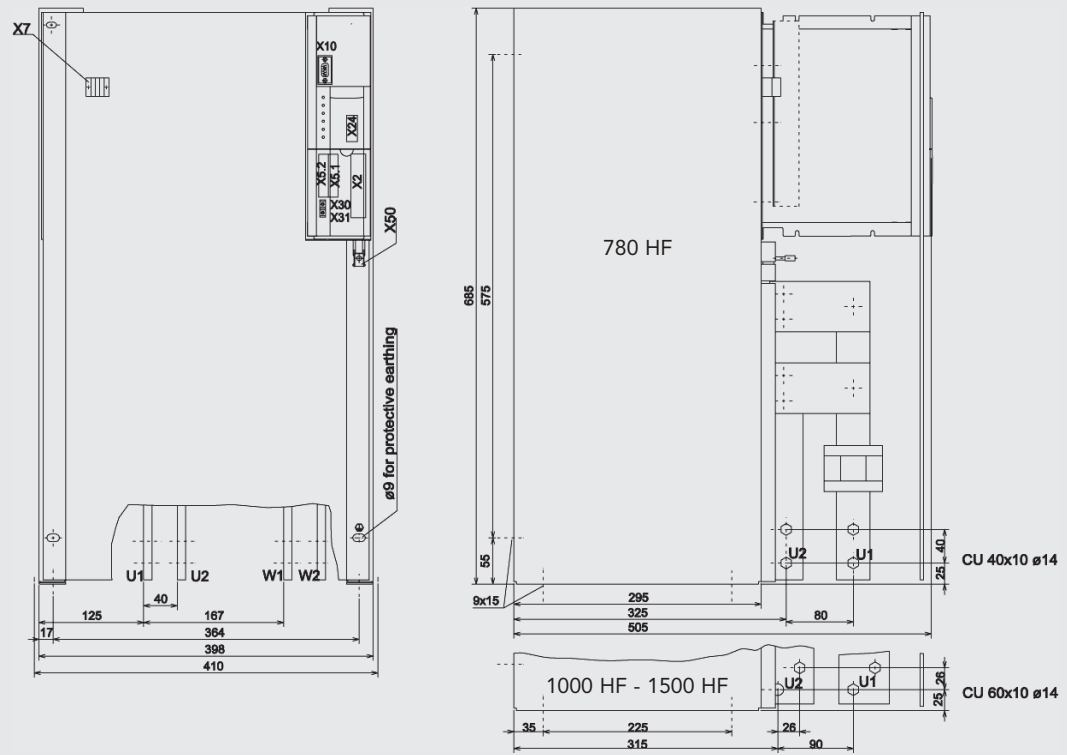
Thyro-P 2P (780 HF, 1000 HF, 1400 HF, 1500 HF)
